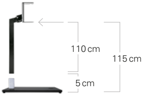
Baseplate and Mount for d&b point source series
