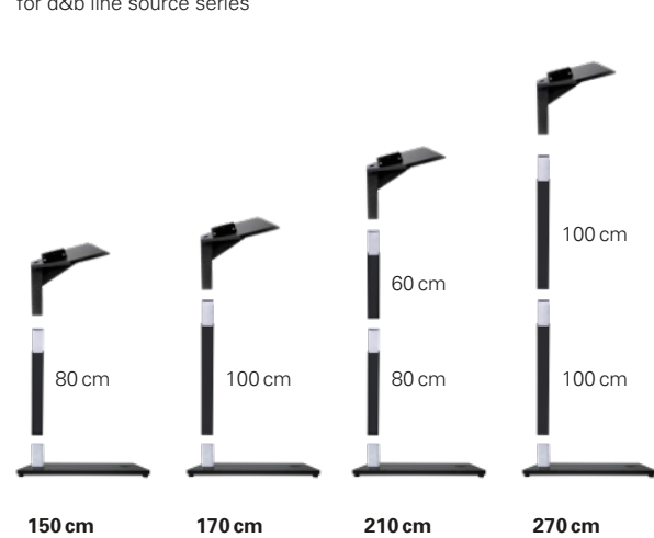
Baseplate and Mount for d&b line source series
