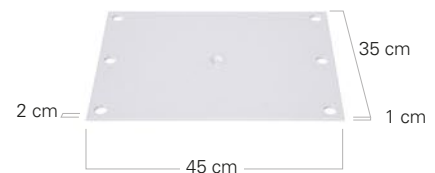
Universal plate
